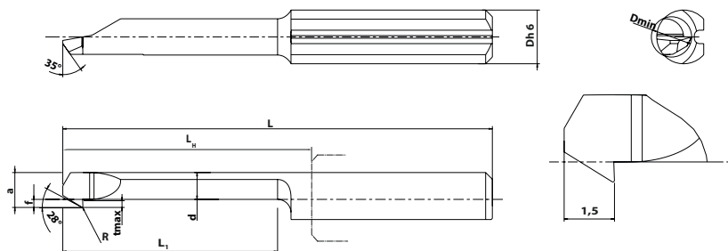
Abmessungen / Dimensions [mm]
