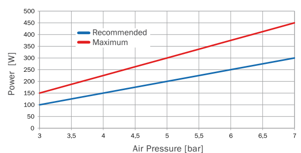
Power/Air Pressure
